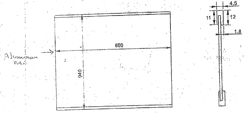
Aluminum bar detail
